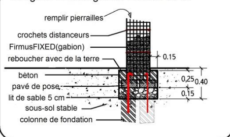
Image 8: Finition gabion FirmusFIXED
