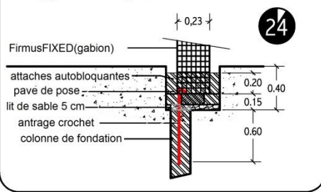
Image 6: Coulage béton
