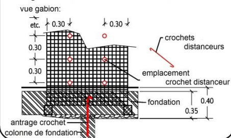
Image 7: Pose crochets distanceurs
